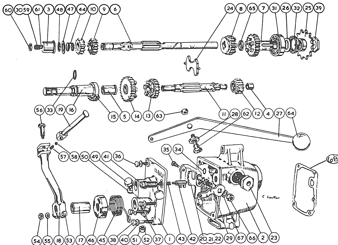
TRANSMISSION — MK III EXP. — MK IV STD.
