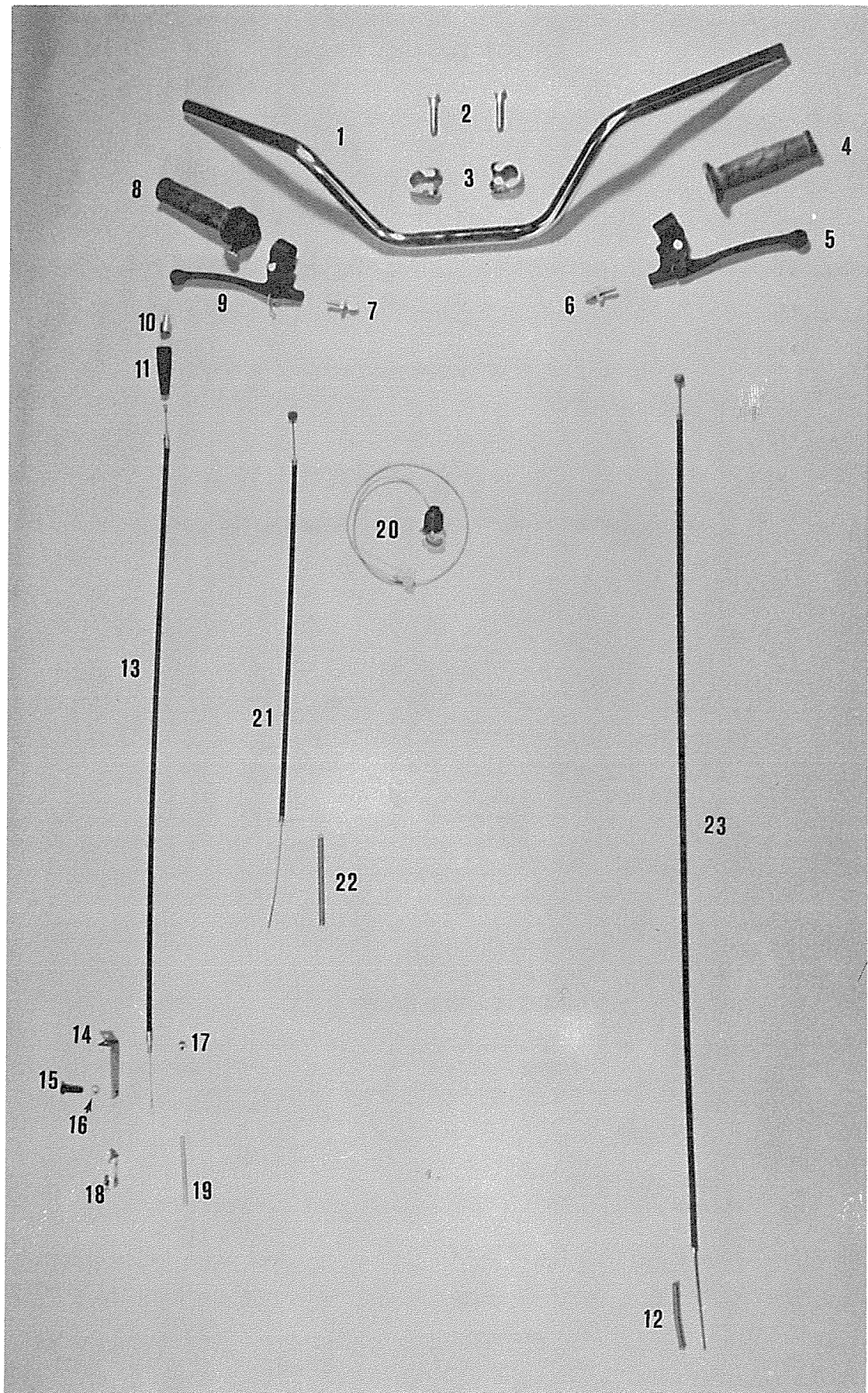
HANDLE BAR ASSEMBLY
