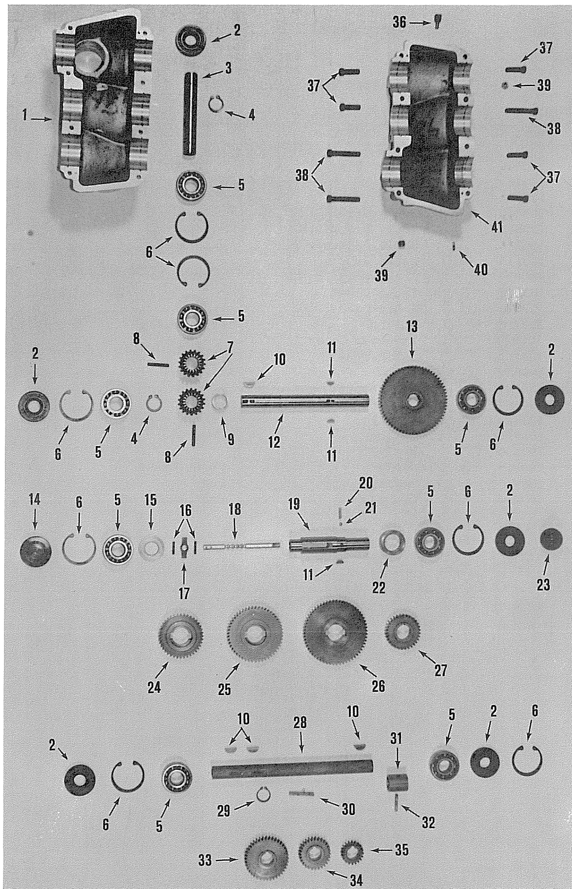
3 SPEED TRANSMISSION
